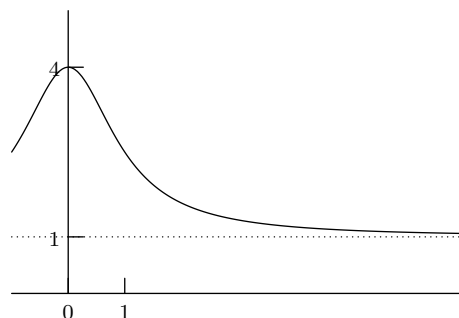
FIGURE 8.3 – Asymptote horizontale
